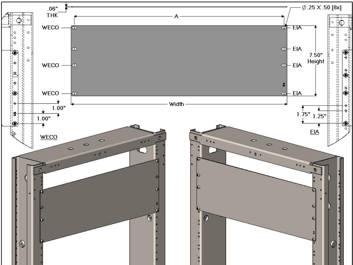
BPU419 - 19.00" Universal Blank Panel
